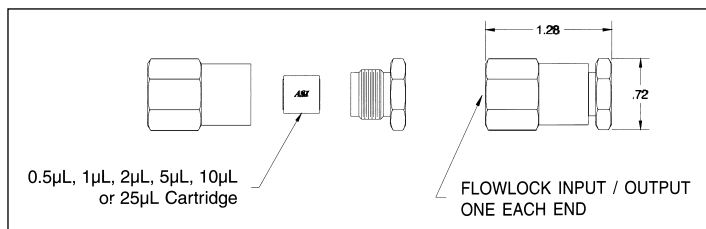
In-Line Assemblies - Port Size: 10-32 CPI (Standard HPLC Fittings for 1/16" Tube)
